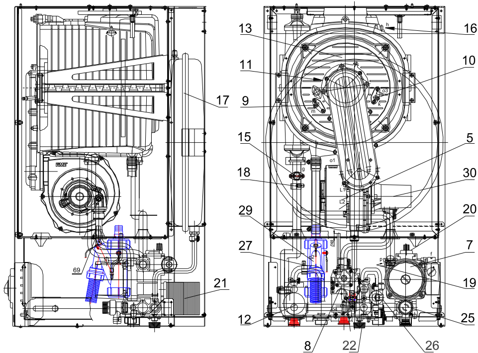
Combi boiler WINDSOR PLUS - 50
